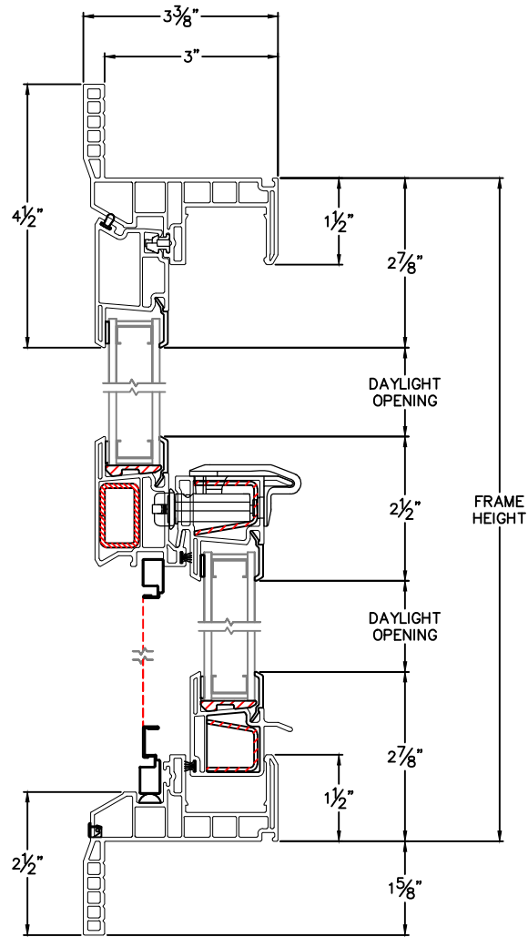
HEAD & SILL
