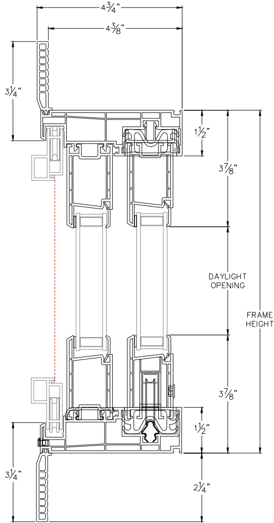
HEAD & SILL
