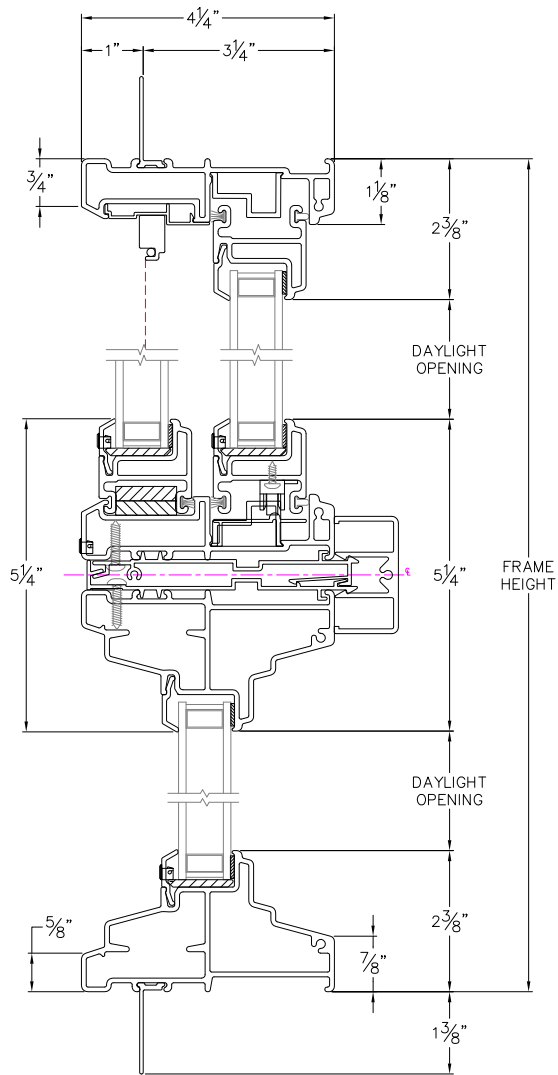
HEAD & SILL
