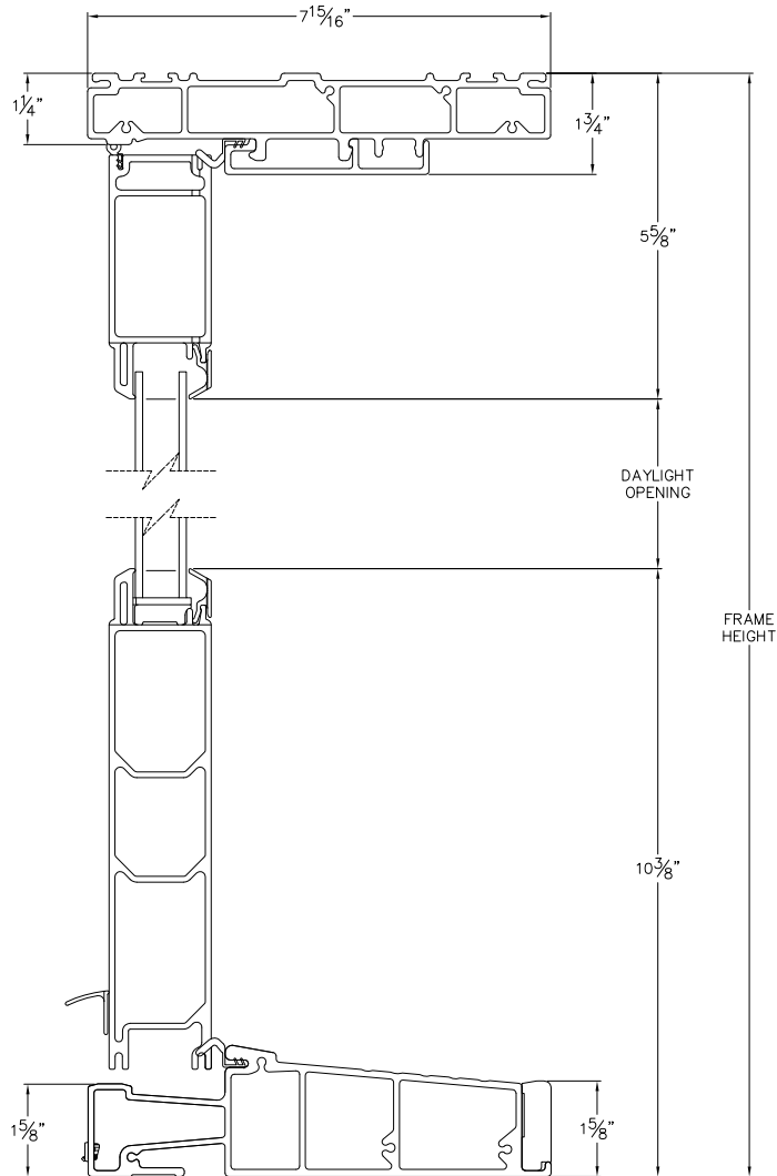
HEAD & SILL
