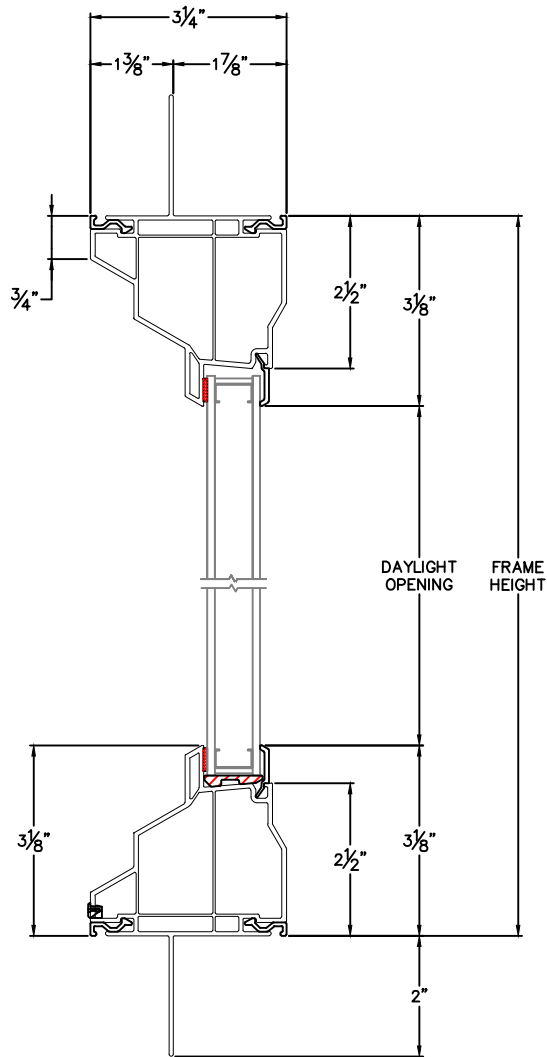
HEAD & SILL
