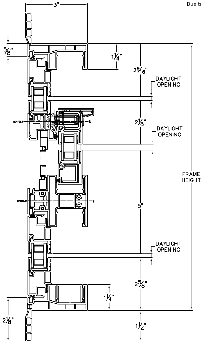
HEAD & SILL
