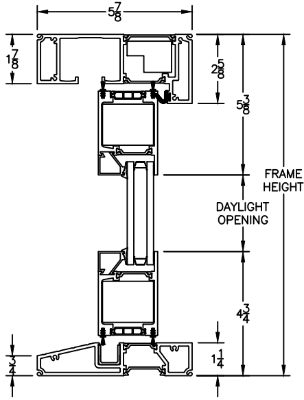
HEAD & SILL
