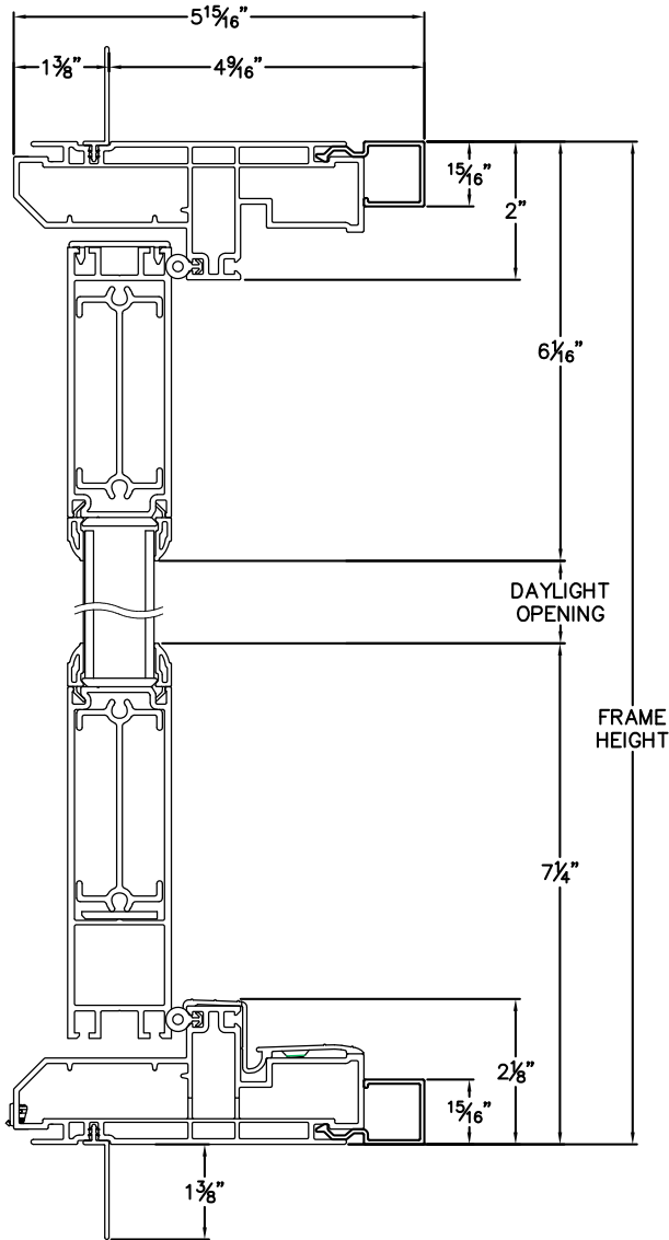
HEAD & SILL
