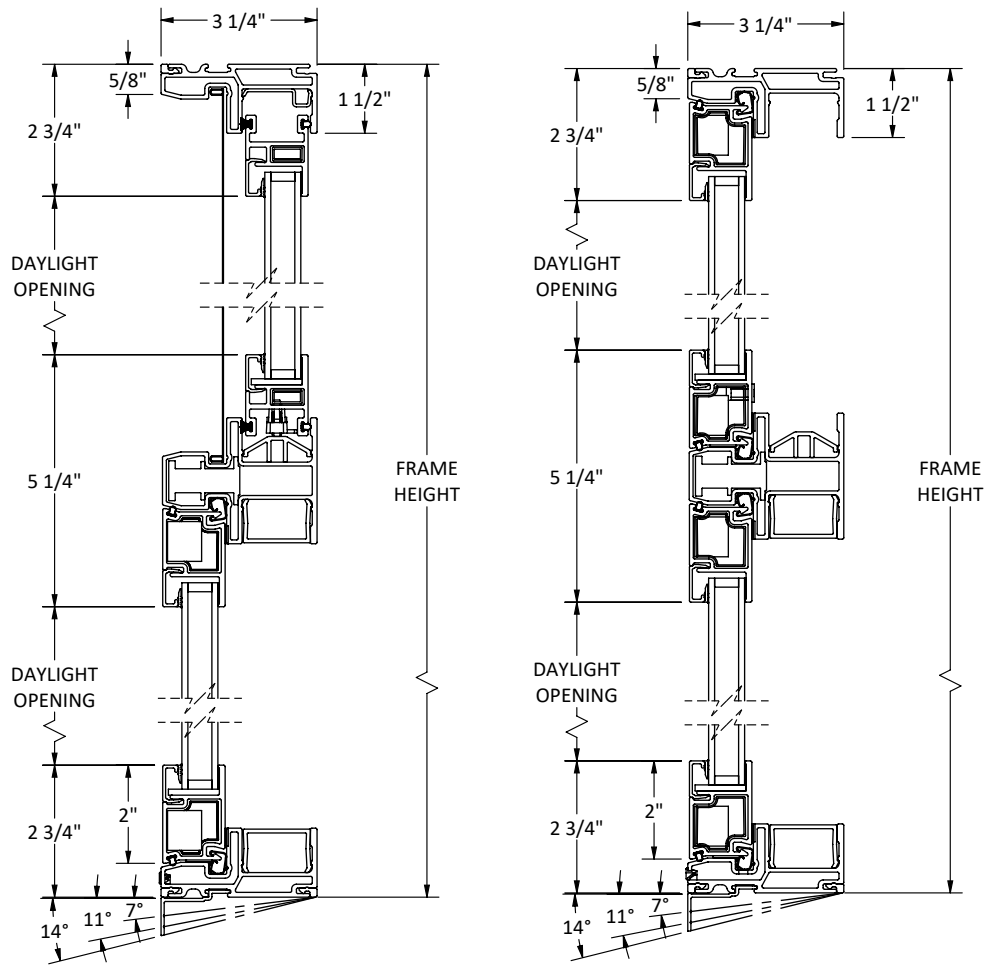
HEAD & SILL
