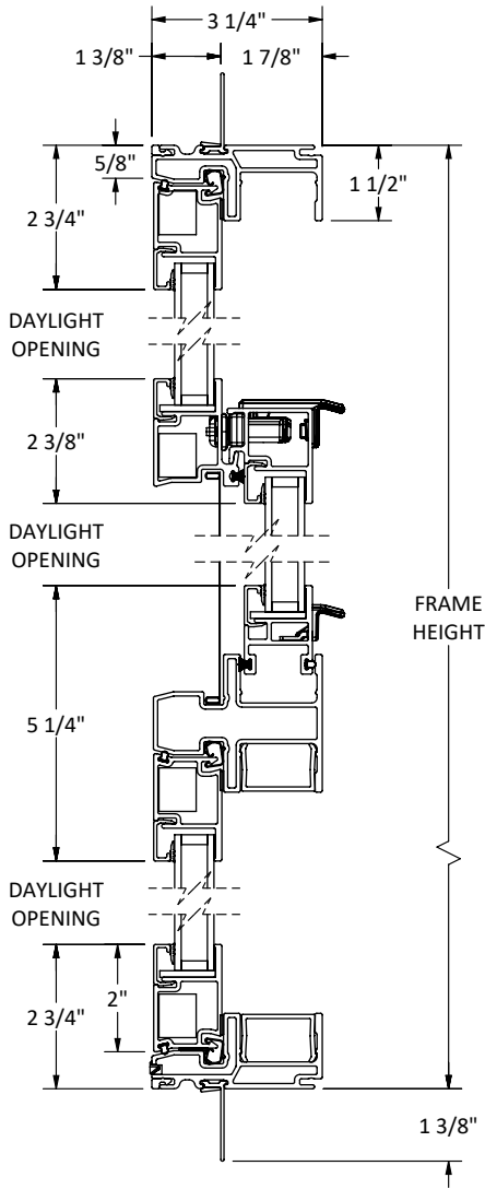
HEAD & SILL
