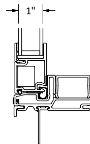
ALTERNATE 1" GLASS I.G.U.
