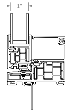
ALTERNATE 1" GLASS I.G.U.
