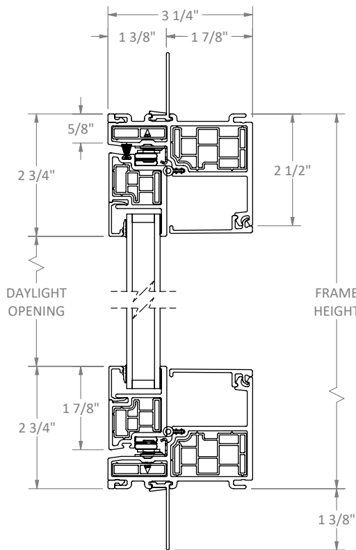
HEAD & SILL
