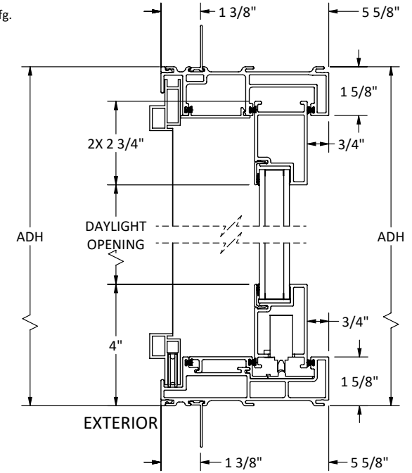
HEAD & SILL
