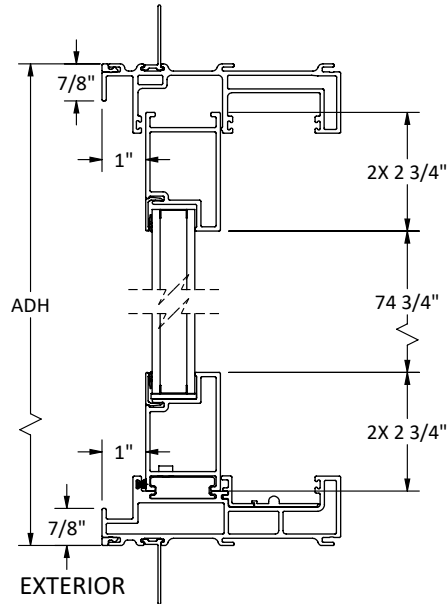
HEAD & SILL
