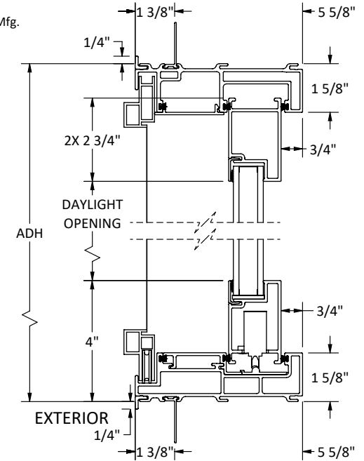
HEAD & SILL
