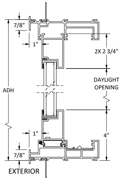
HEAD & SILL
