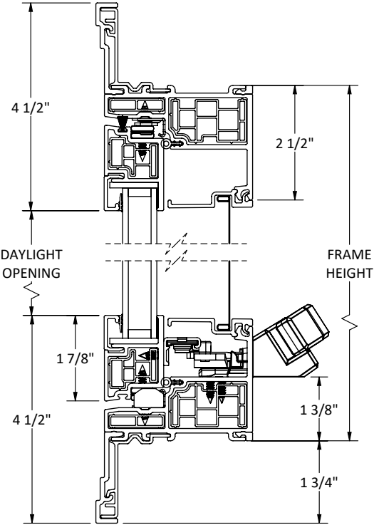
HEAD & SILL
