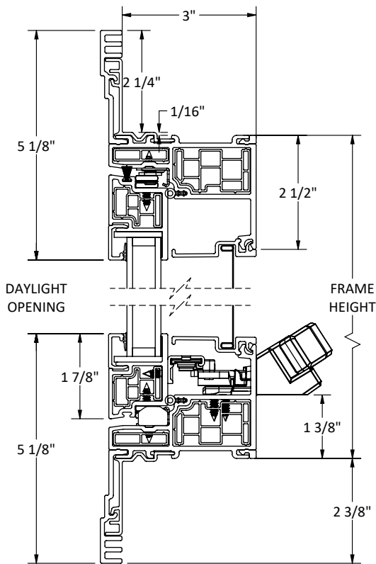
HEAD & SILL
