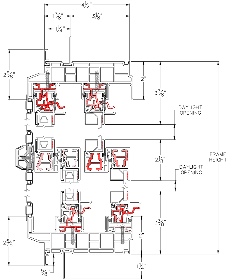
HEAD & SILL
