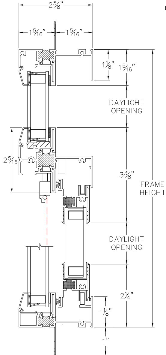
HEAD & SILL
