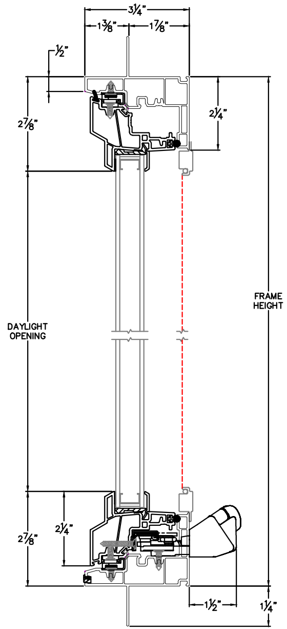
HEAD & SILL
