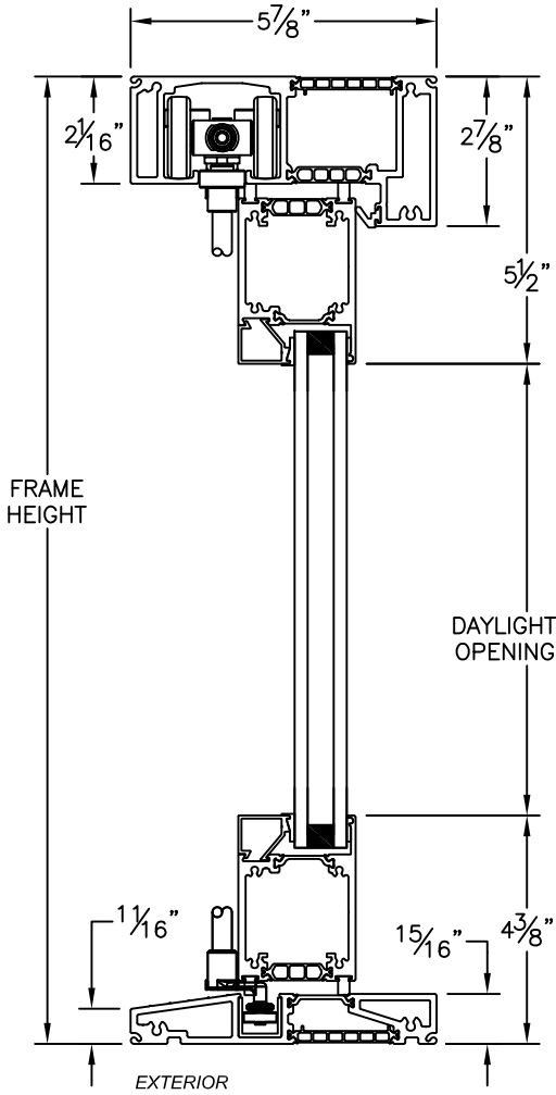
HEAD & SILL
