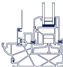
1 3/8" Mounting Fin Set-back w/ Stucco Key*
