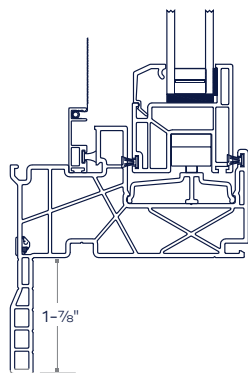
1 7/8" Contoured Flush Fin*
