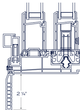
2 1/4" Contoured Z-Bar
