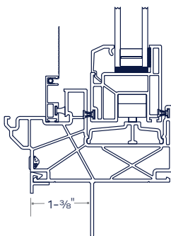
1 3/8" Mounting Fin Set-back w/ Stucco Key*
