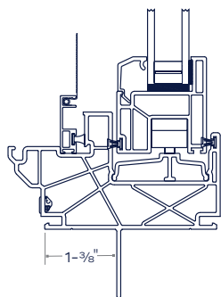
1 3/8" Mounting Fin Set-back
