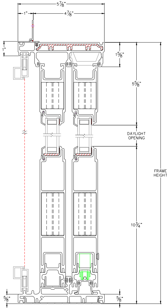
HEAD & SILL
