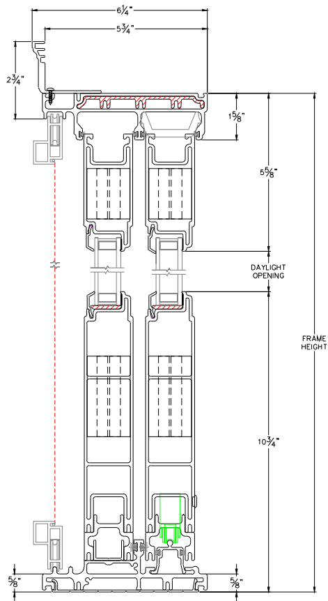
HEAD & SILL
