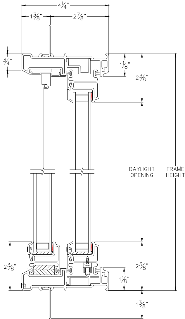
HEAD & SILL
