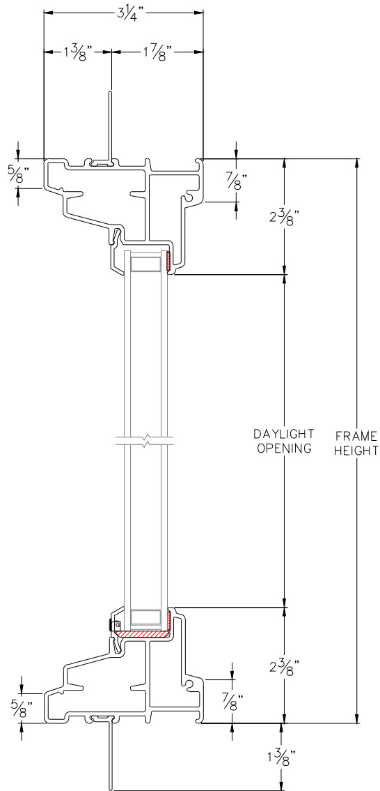
HEAD & SILL
