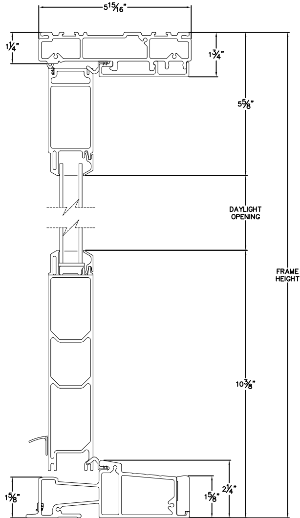
HEAD & SILL
