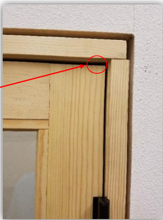
Gap between the Top of the Door Panel and the Frame Head
