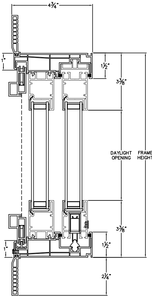
HEAD & SILL
